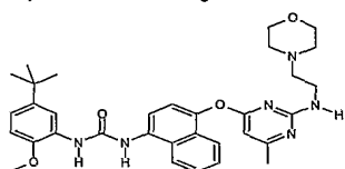
1-(5-tert-Butyl-2-methoxy-phenyl)-3-{4-[6-methyl-2-(2-morpholin-4-yl-ethylamino)-pyrimidin-4-yloxy]-naphthalen-1-yl}-urea;
